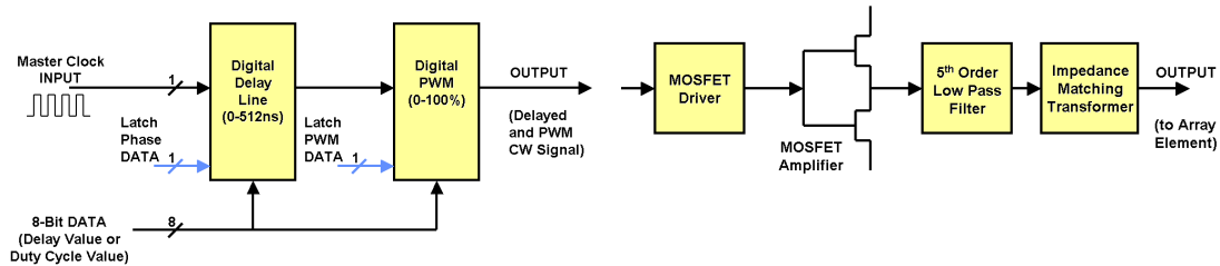
FIGURE 6. Digital (left) and analog (right) block diagrams of array driving electronics (one channel).
