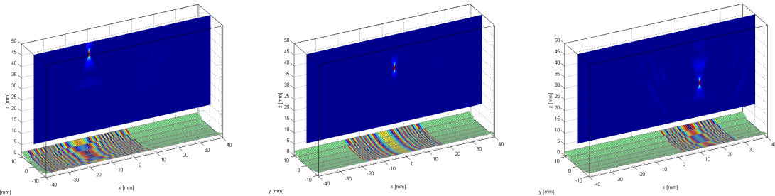
FIGURE 4. Longitudinal Steering using Subapertures, and Depth Focusing using variable-size Subapertures to maintain a fixed f-number and eliminate off-axis steering gain loss.
