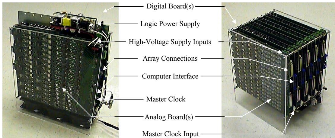
FIGURE 7. 20 Channel High-Power System (left) and 320 Channel Low-Power System (right).
