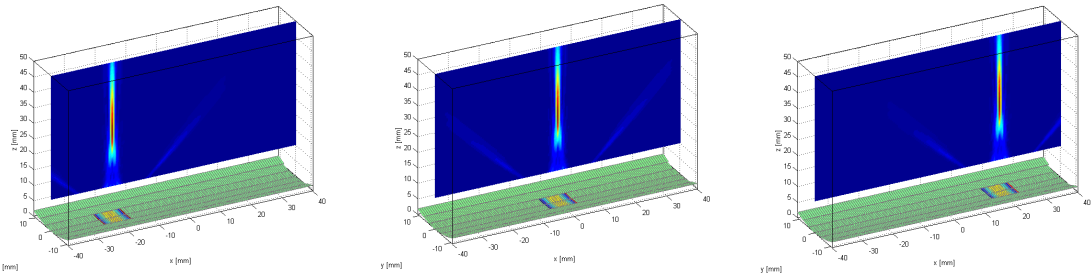
FIGURE 5. Linear Mechanical Imaging Function replacement with Electronically-controlled Imaging using Imaging Subapertures (2D Image = assembly of 1D RF-lines; 2-4 frames/second expected).
