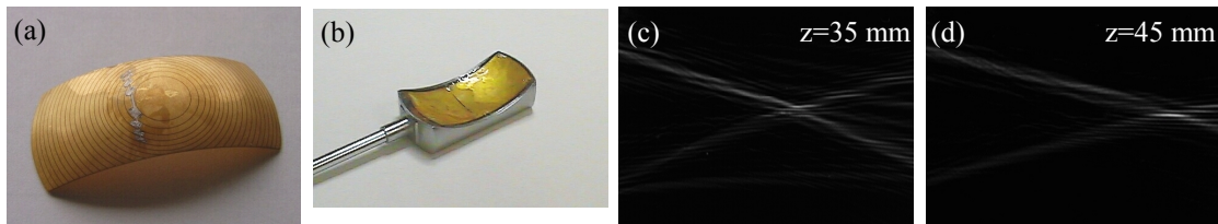
FIGURE 3. (a) 20-Ring Annular Array Crystal, (b) Transducer Assembly, and (c-d) Qualitative Evaluation of Focusing Ability of Array using Schlieren Imaging.
