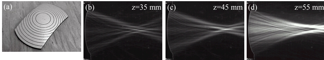
FIGURE 1. (a) 9-Ring Annular Array Crystal, and (b-d) Qualitative Evaluation of Focusing Ability of Array using Schlieren Imaging.
