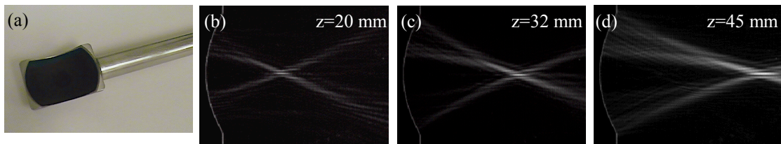
FIGURE 2. (a) 17-Ring Annular Array Transducer Assembly, and (b-d) Qualitative Evaluation of Focusing Ability of Array using Schlieren Imaging.
